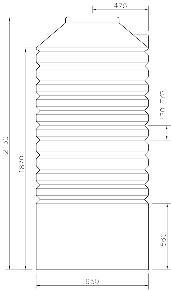
FRONT VIEW 1:50
