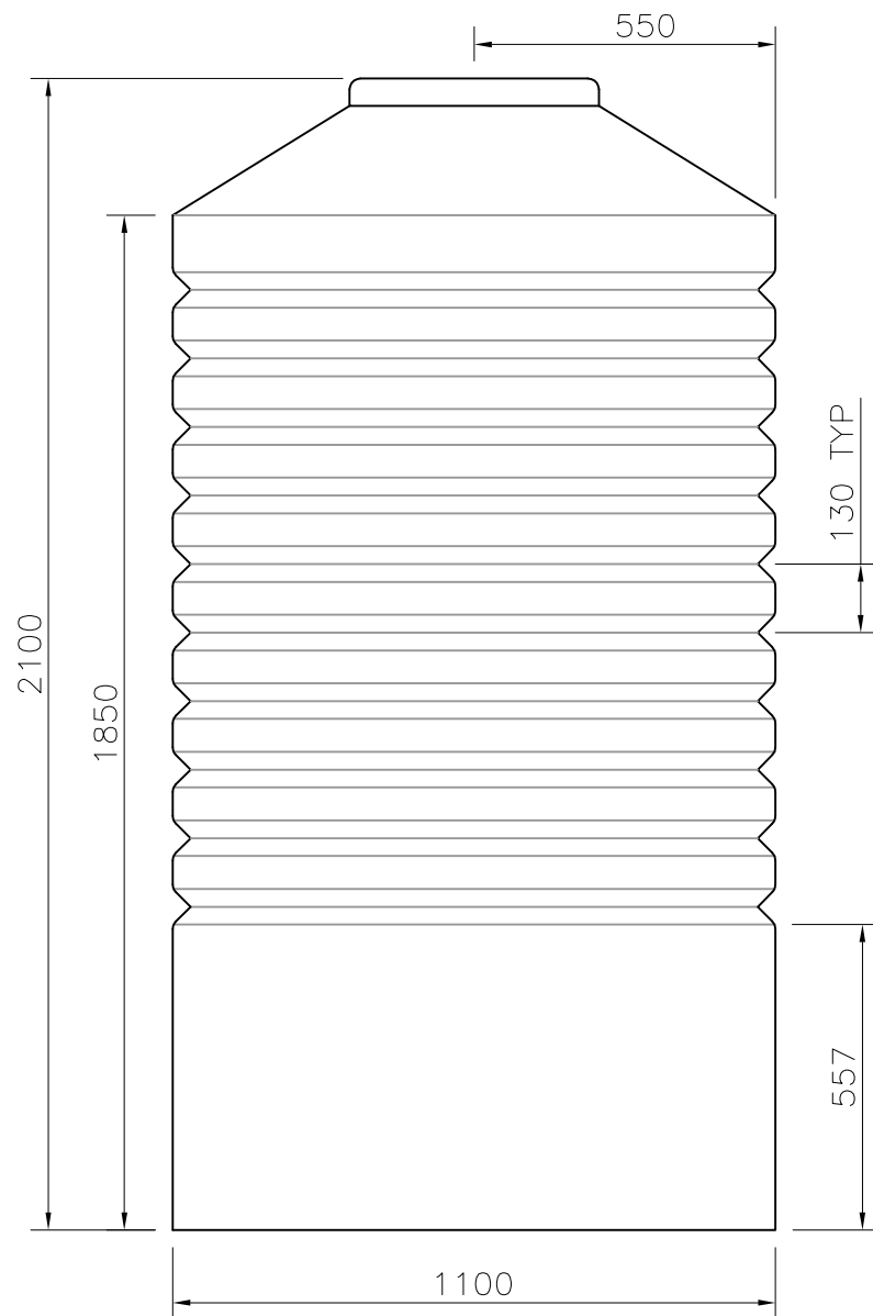
FRONT VIEW 1:50
