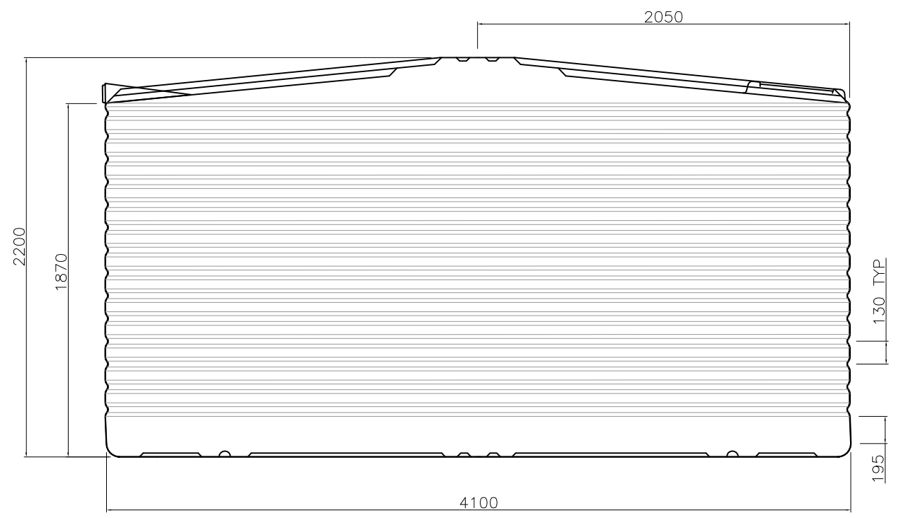
FRONT VIEW 1:50
