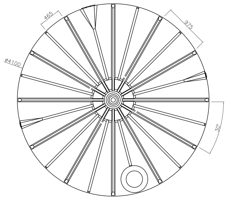
TOP VIEW 1:50
