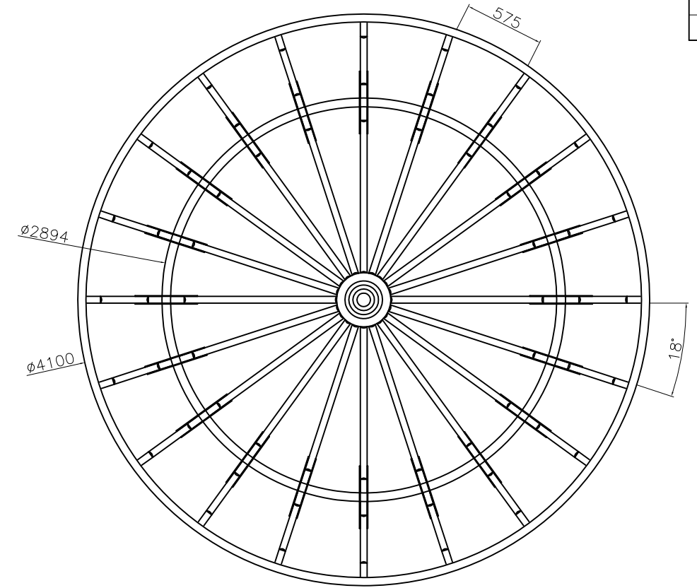
BOTTOM VIEW 1:50
