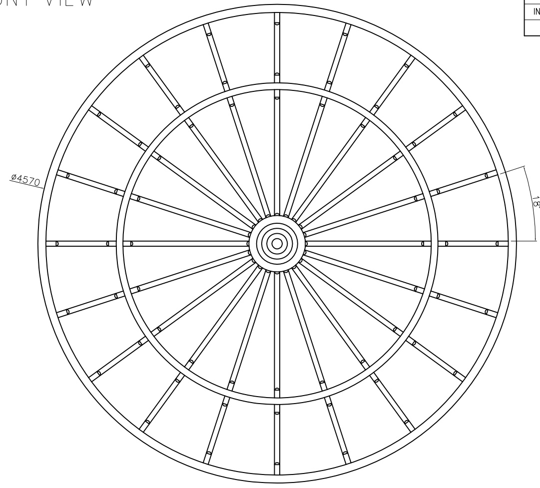
BOTTOM VIEW
